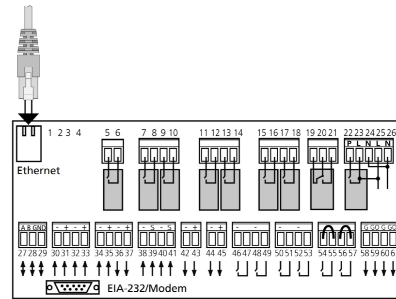
Fig. 21 Ethernet cable from INSIDE Connect to GOLD IQlogic control card.
