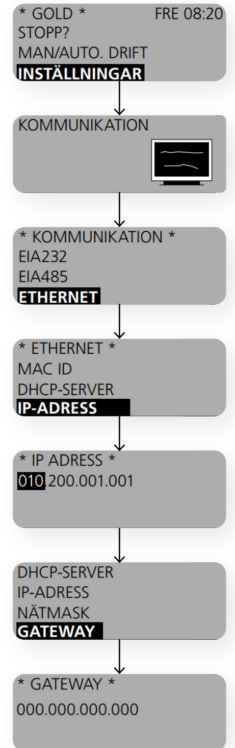
Fig. 22. Network settings in GOLD AHU, version C or D.
