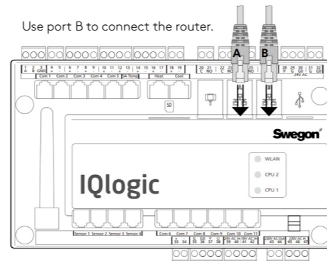
Figure 17. Ethernet cable from INSIDE Connect to GOLD IQlogic control card.
